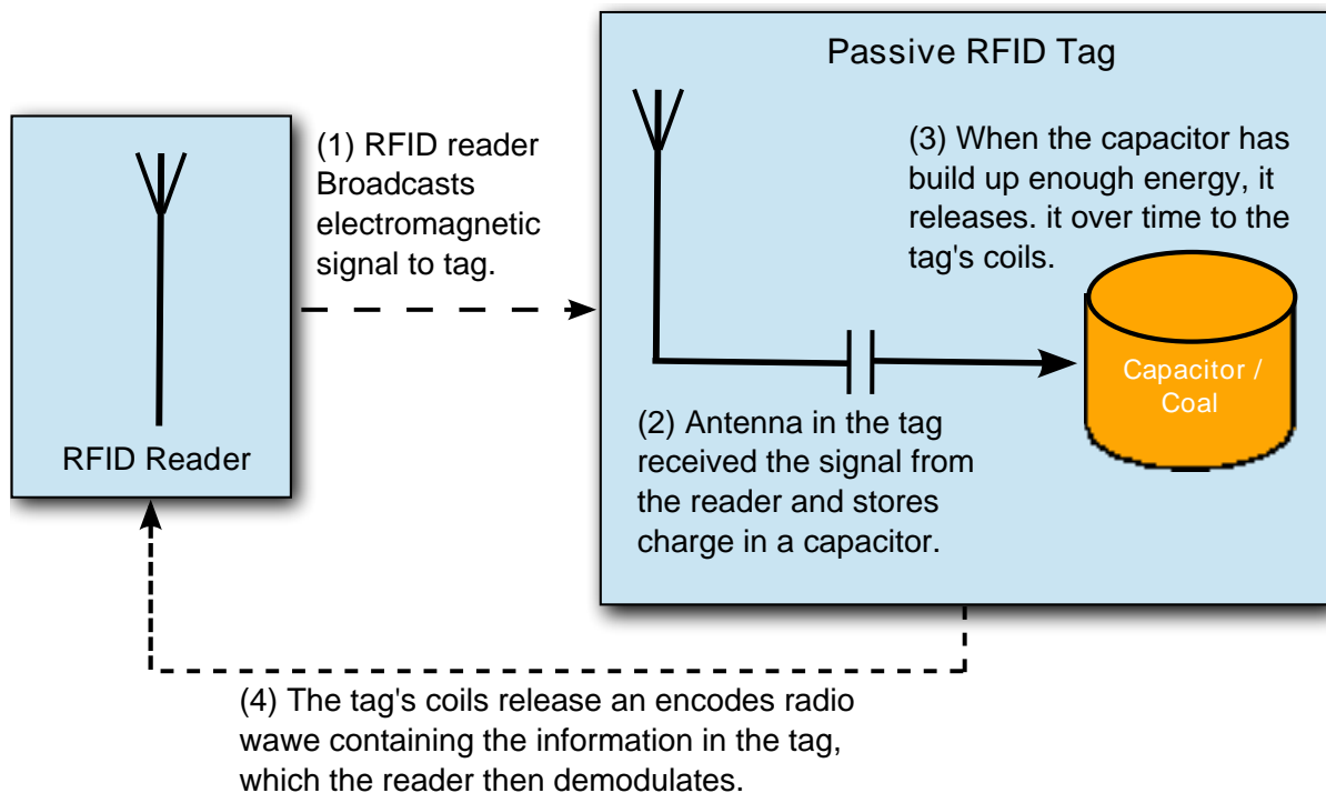
Figure 1.4. RFID Example
