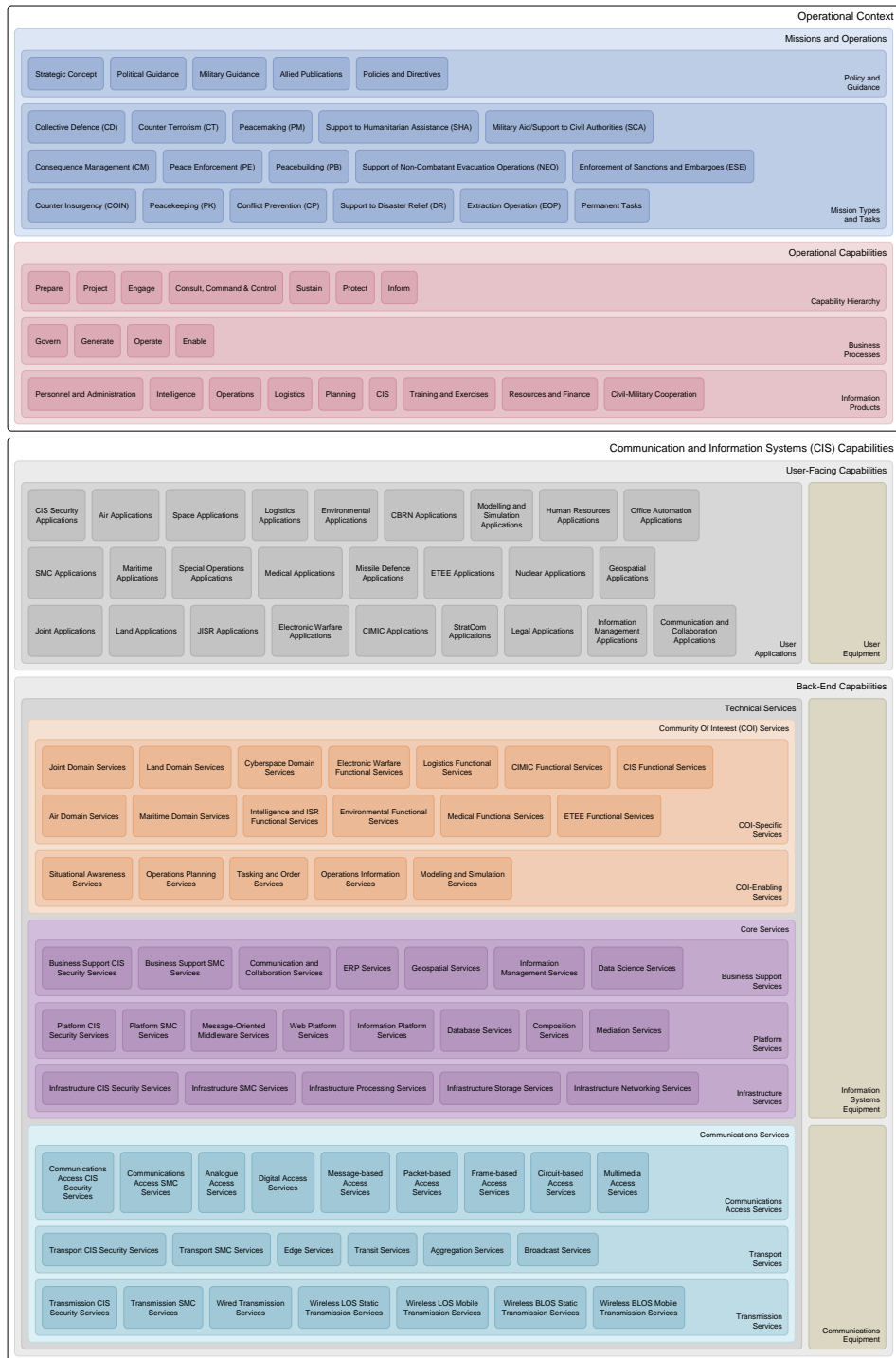
Figure 7.1. C3 Taxonomy
